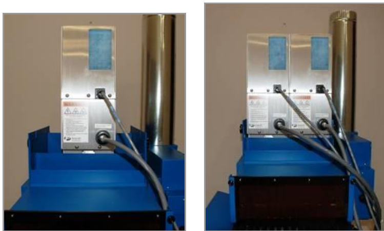
Figure 8. Irradiator Cable Connections
