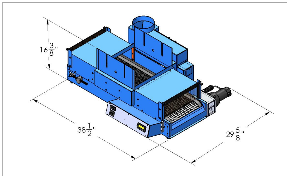
Figure 26. UVCS 39 Dimensions
