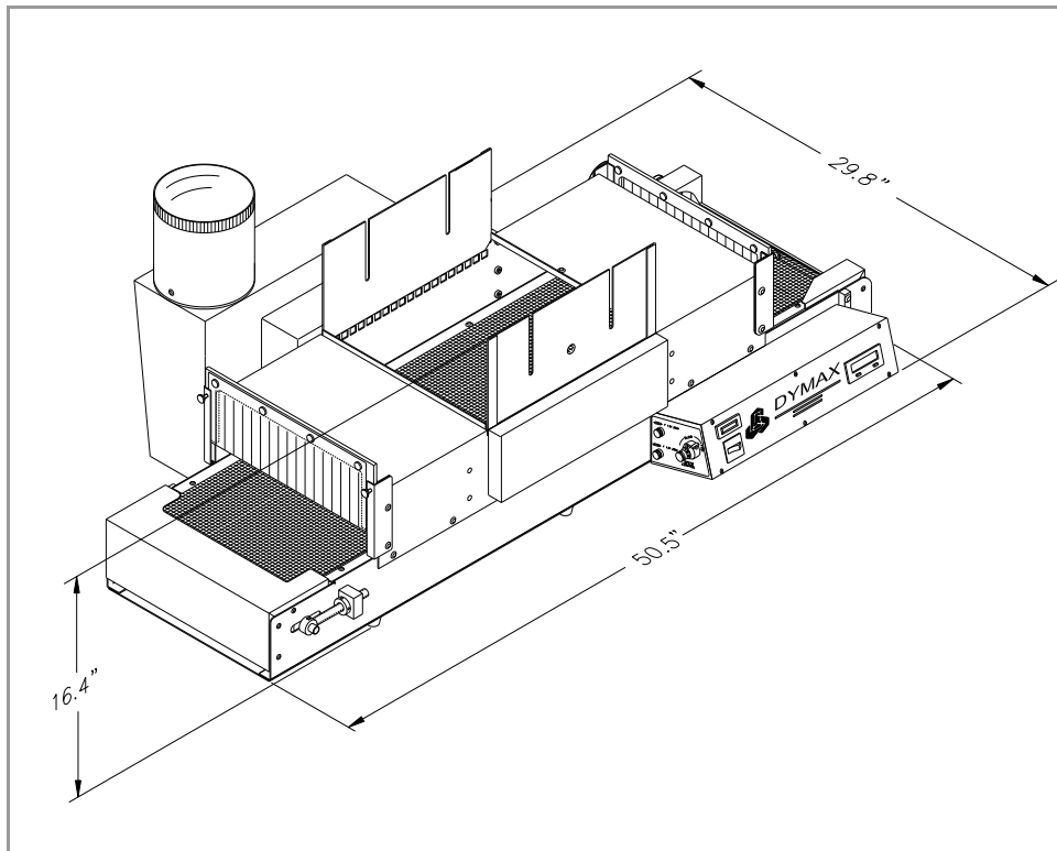
Figure 25. UVCS Version 2.0 Dimensions
