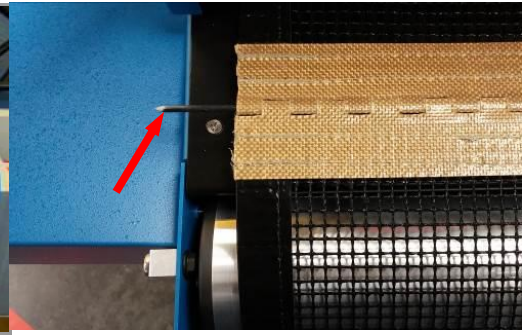
Figure 21. Fiberglass Rod
