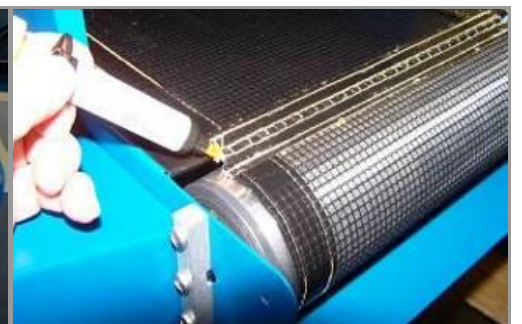
Figure 23. Applying Adhesive
