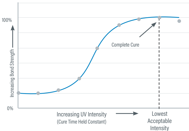
Figure 2. UV Curing Profile (Cure Time Held Constant)
