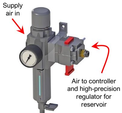
Figure 4. Filter Regulator
